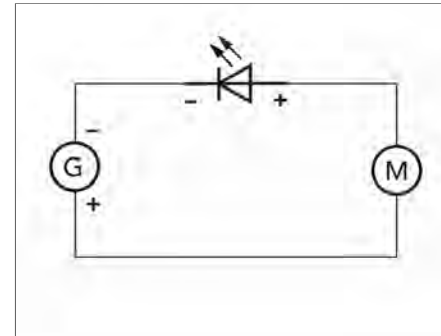
Schaltplan: Generator - Motor - LED
